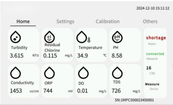
Fig.5 Displays the interface
