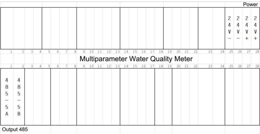
Fig.13 Wiring diagram of multi-parameter water analyzer 485
