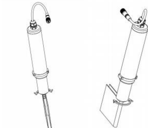
Fig.12 Polishing of Membraneless Dual Platinum Ring sensor
