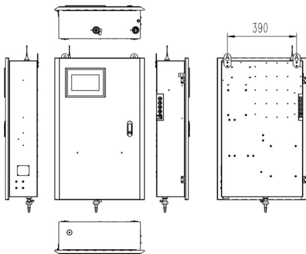
Fig.3 View of the equipment in all directions
